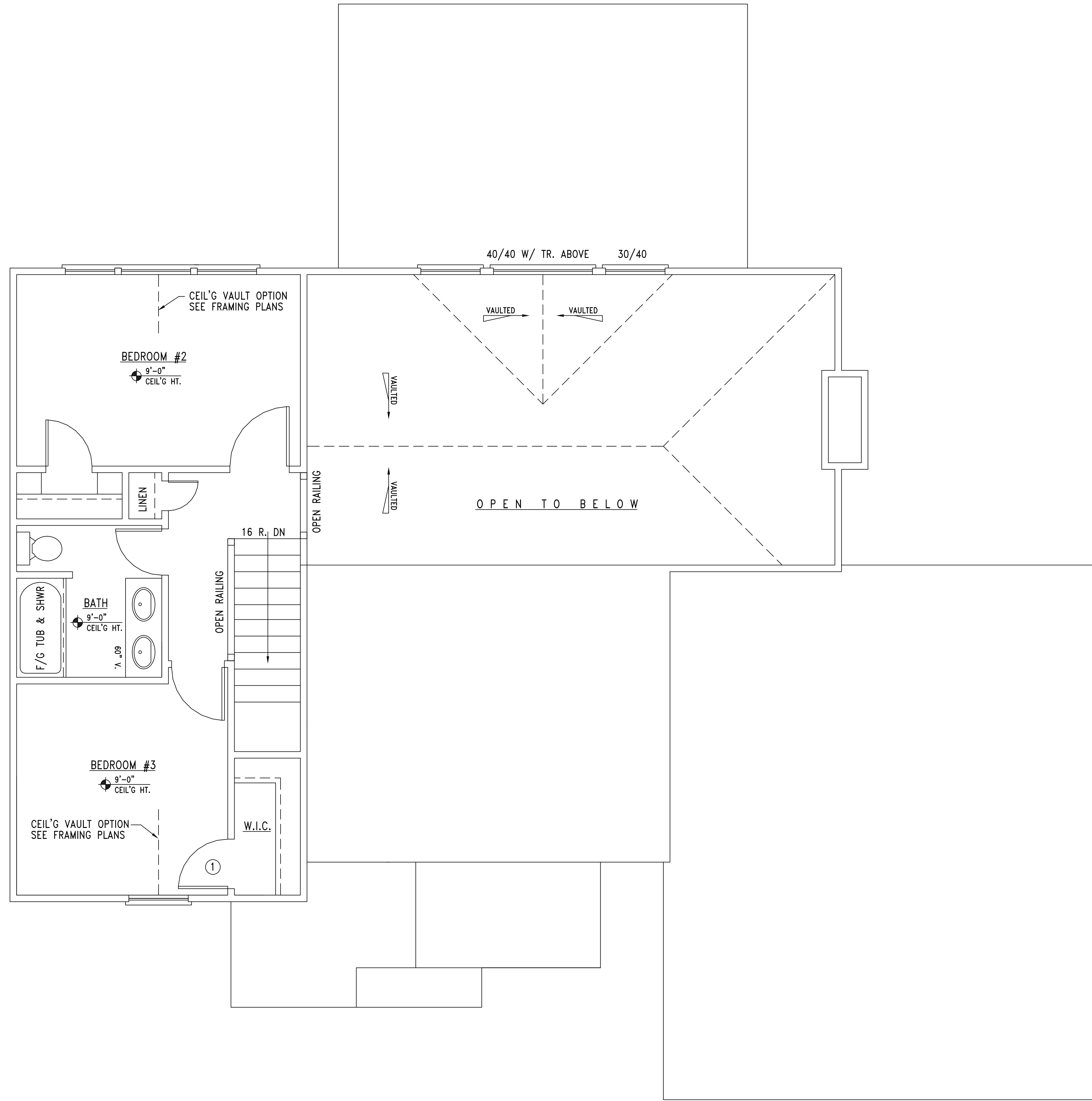
A UPPER LEVEL FLOOR PLAN
