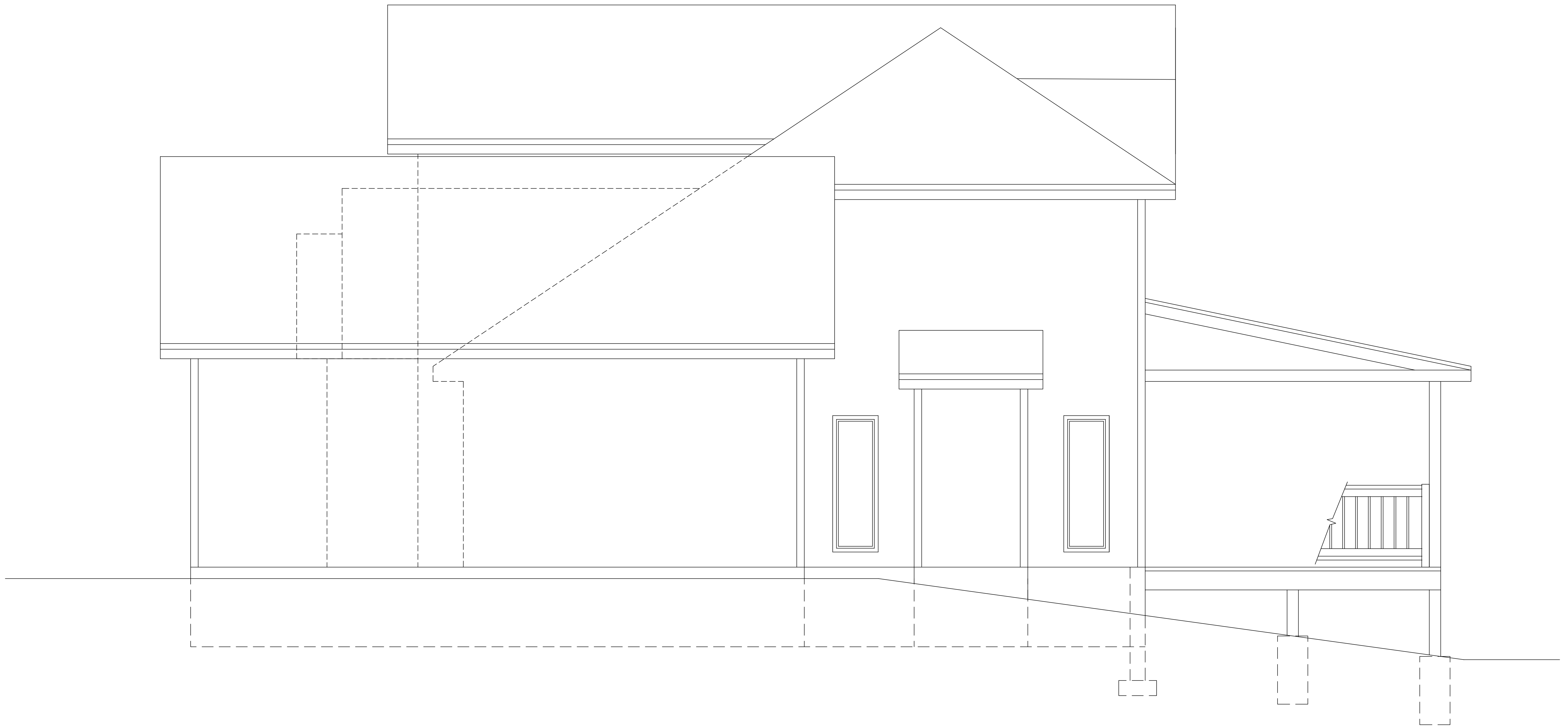
B SIDE ELEVATION
