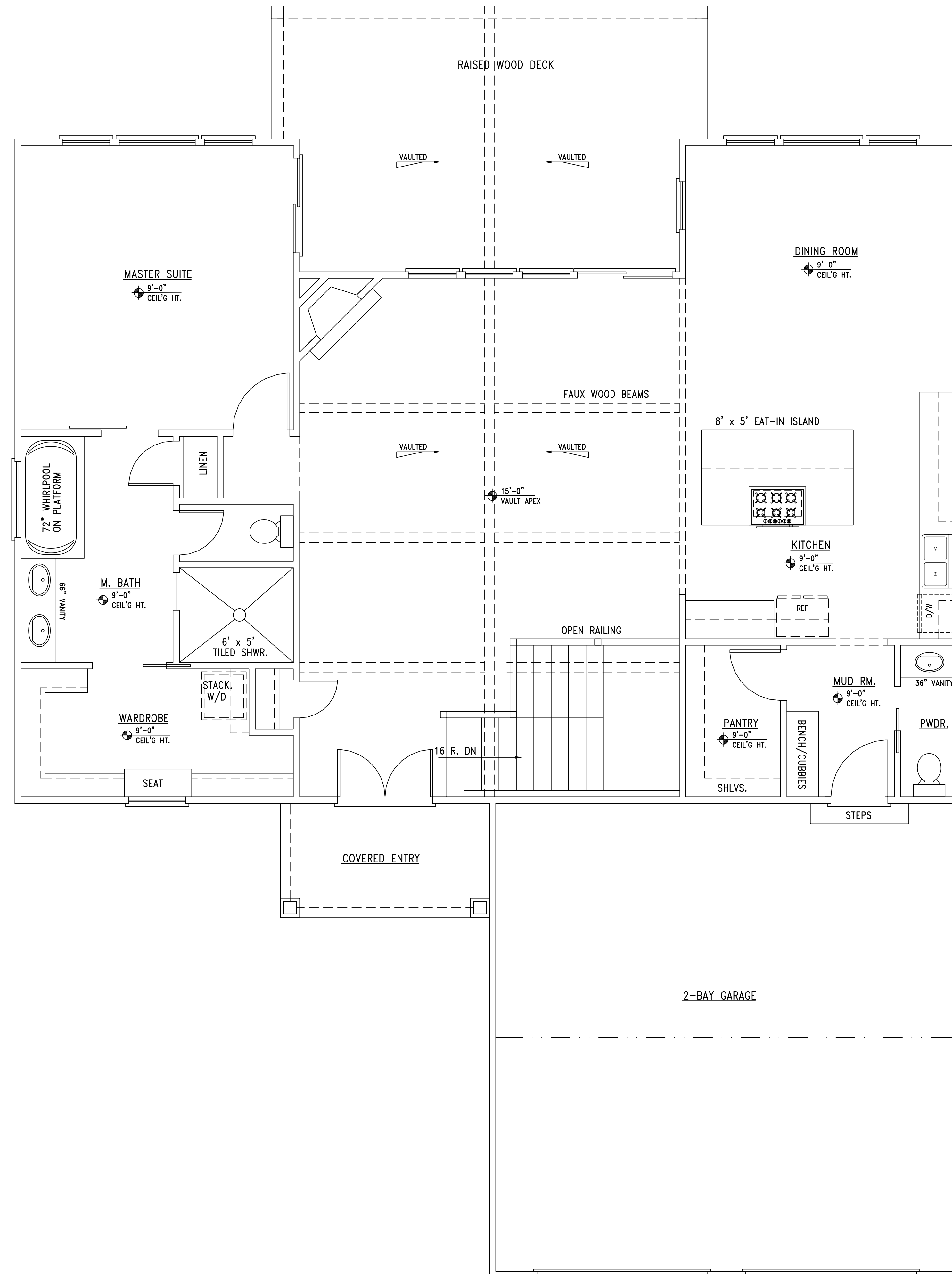
A MAIN LEVEL FLOOR PLAN
