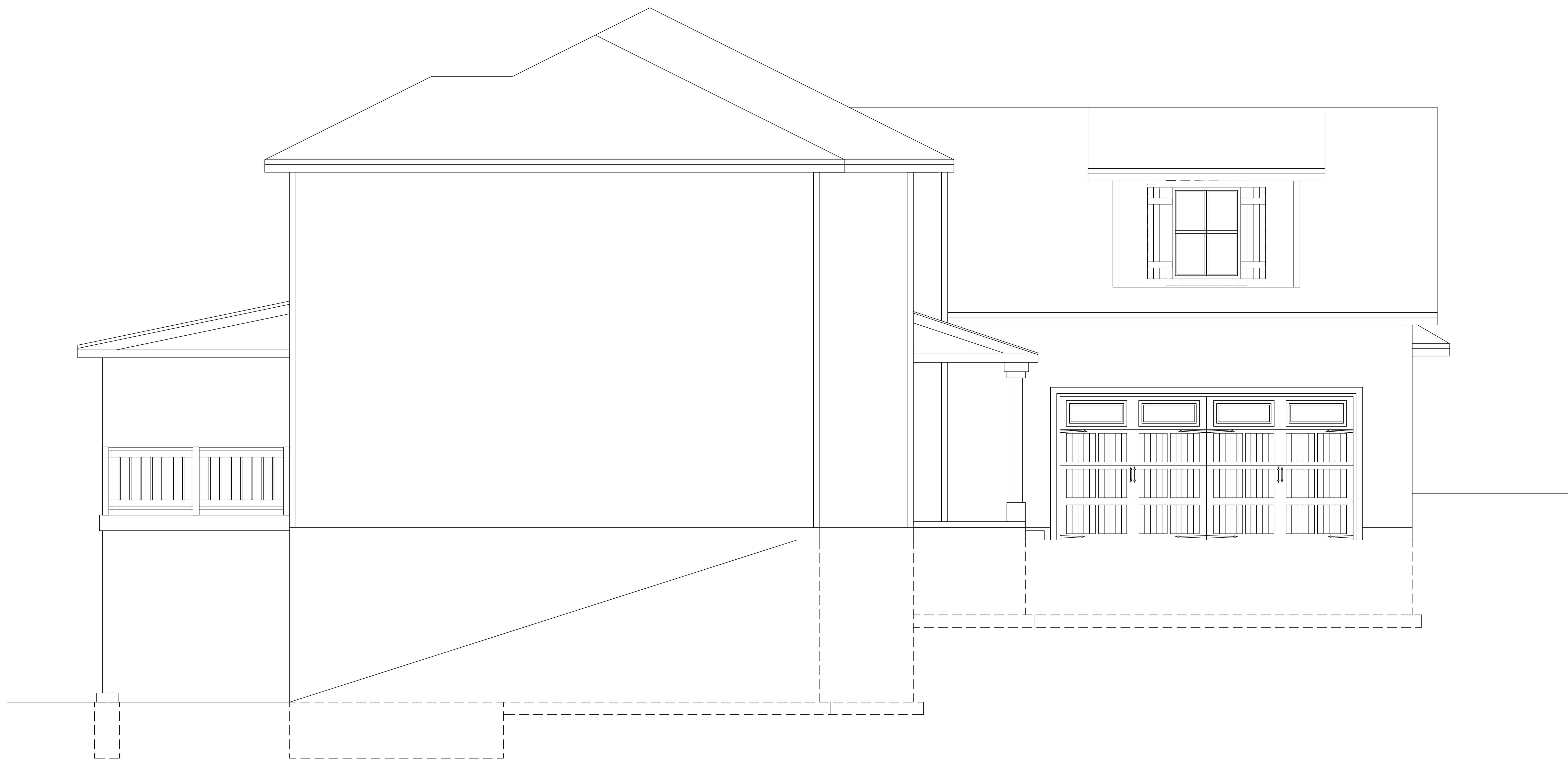
D SIDE ELEVATION
